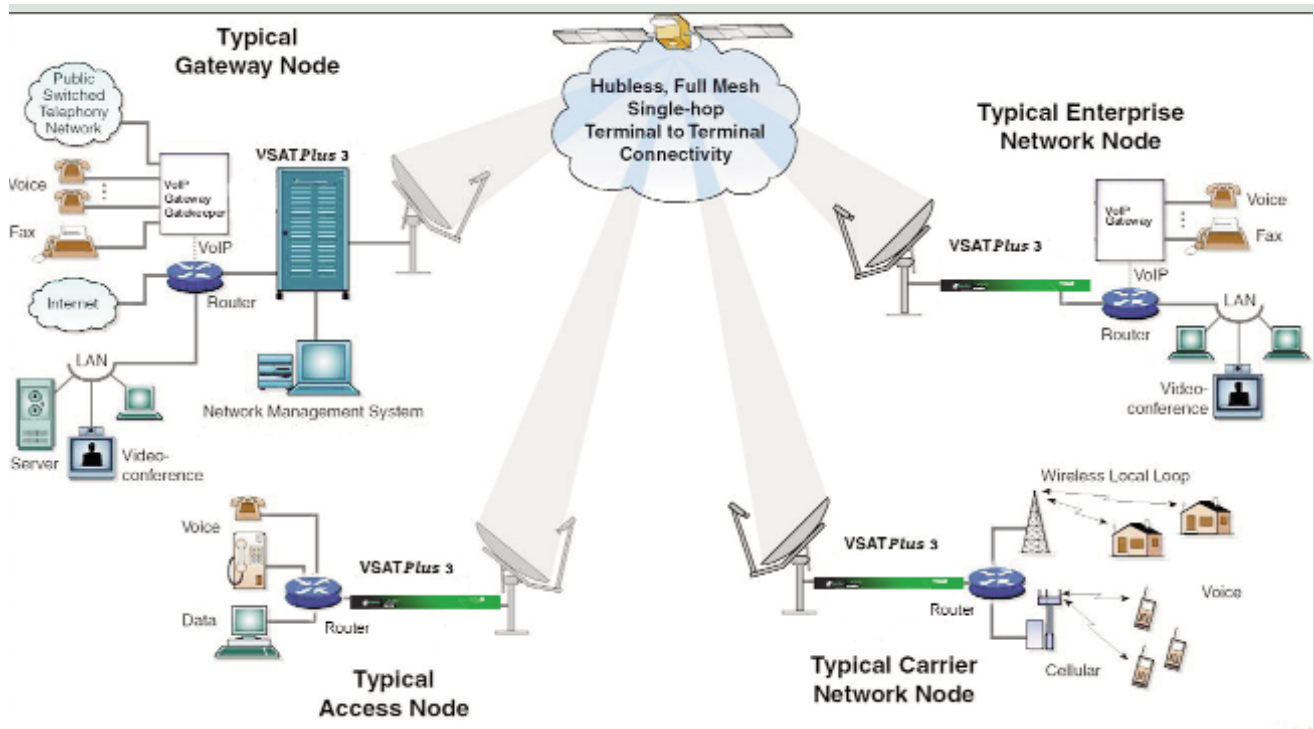
Figure 2 Typical VSATPlus 3 configuration.
